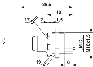
Dimensional drawing
